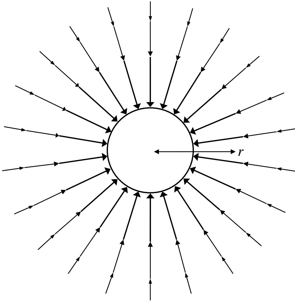
Figure 1. A two-dimensional representation of the gravitational flow of Newtonian-Lorentzian, inertial-electromagnetic space into all matter. The acceleration of the flow at any height, r , is GM/r^2 and the velocity is \sqrt{2GM/r} . The acceleration explains the ballistic effects of gravity; the velocity explains the electromagnetic (relativistic) effects.
